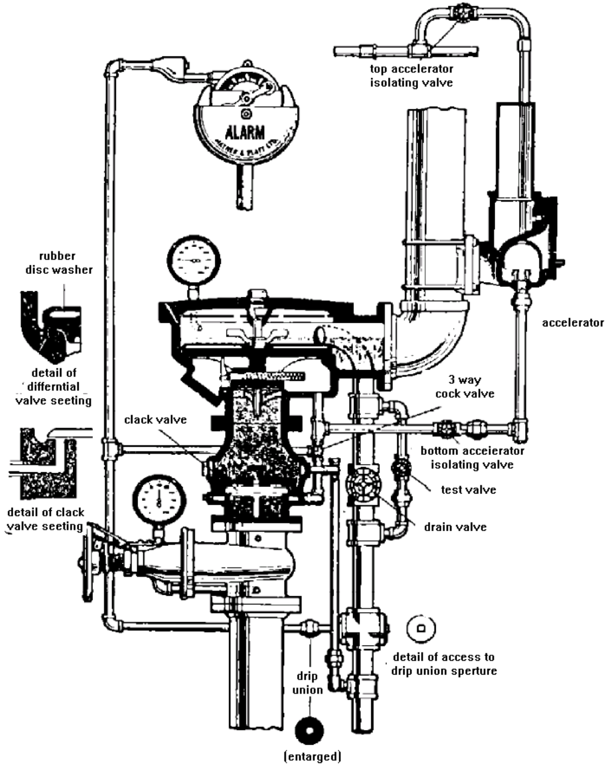
DIAGRAM OF THE CONTROL VALVES OF A TYPICAL ALTERNATE SPRINKLER INSTALLATION Fig. 1
