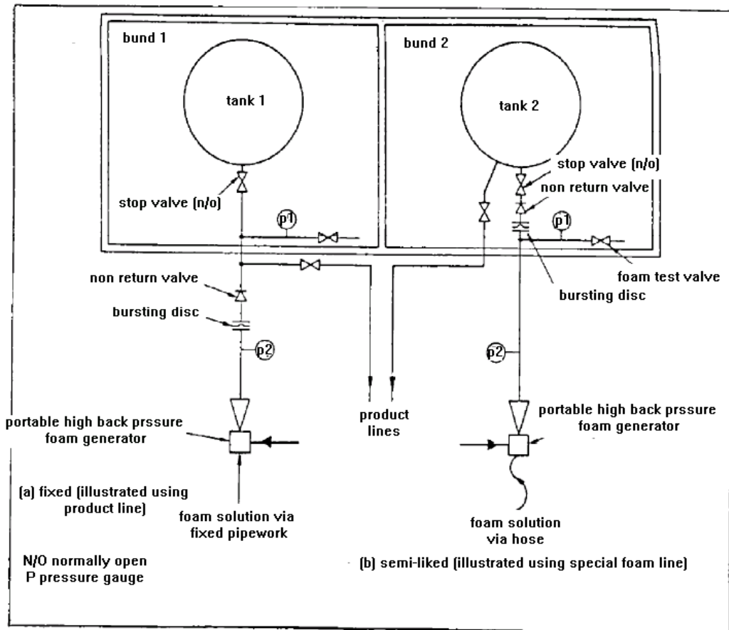
TYPICAL FIXED AND SEMI-FIXED SUBSURFACE SYSTEMS
