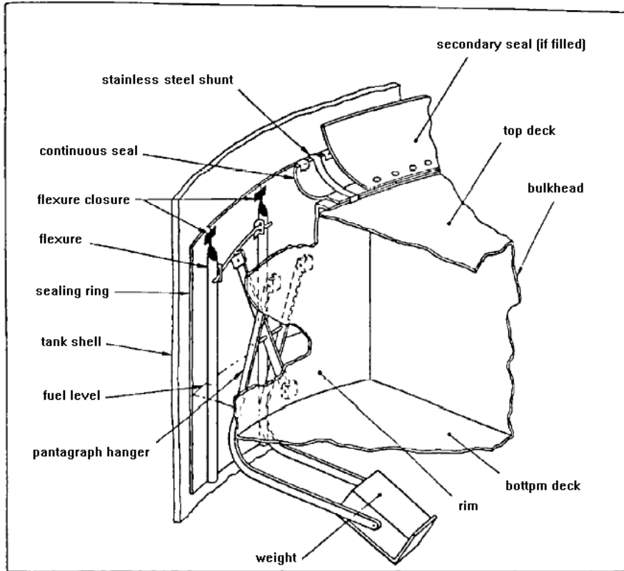
TYPICAL PANTOGRAPH SEAL Fig. 1
