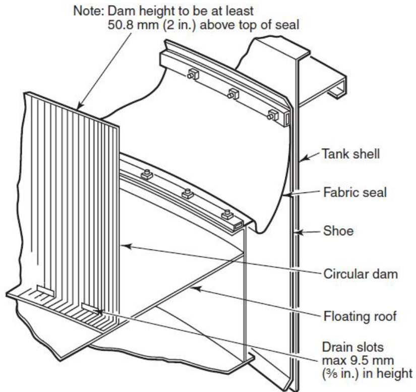
TYPICAL FOAM DAM FOR FLOATING ROOF TANK PROTECTION Fig. 2
