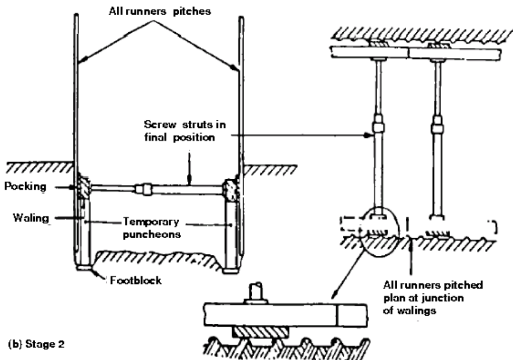
TRENCH EXCAVATION USING STEEL TRENCH SHEETS AS RUNNERS
