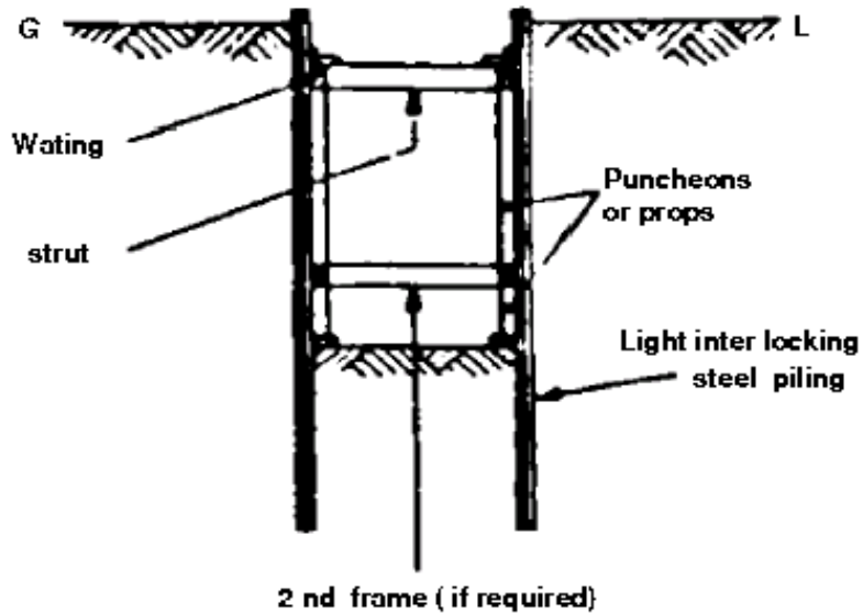
WIDE AND DEEP TRENCH USING STEEL SHEET PILING
