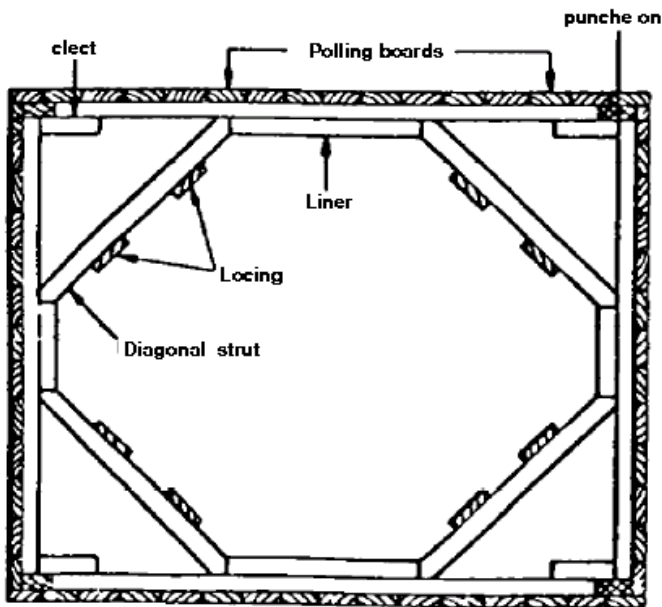
METHOD OF EXCAVATING ISOLATED PITS AND SHAFTS
