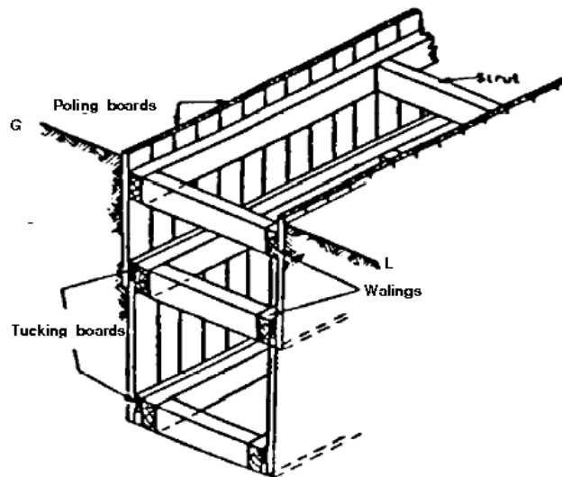
CLOSE POLING WITH TRUCKING FRAMES
