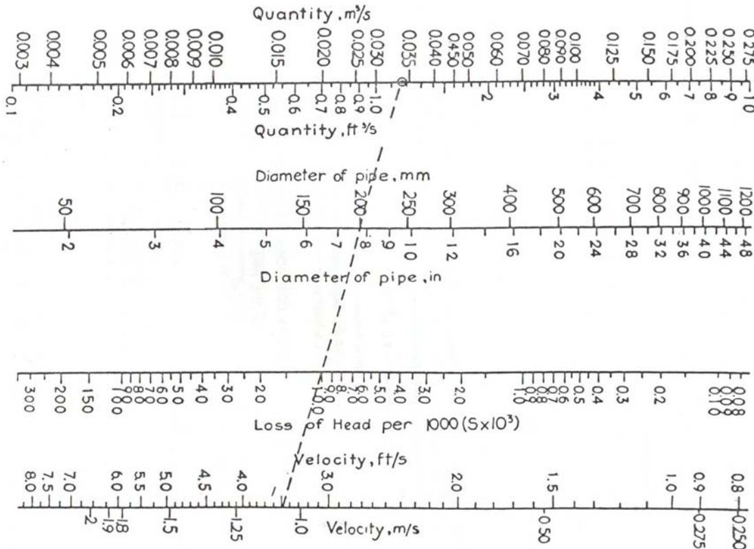
FLOW IN OLD CAST-IRON PIPES (HAZEN-WILLIAMS C = 100)
