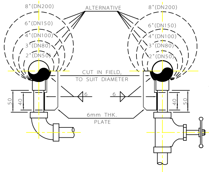
No.1 PERPENDICULAR BRACE
