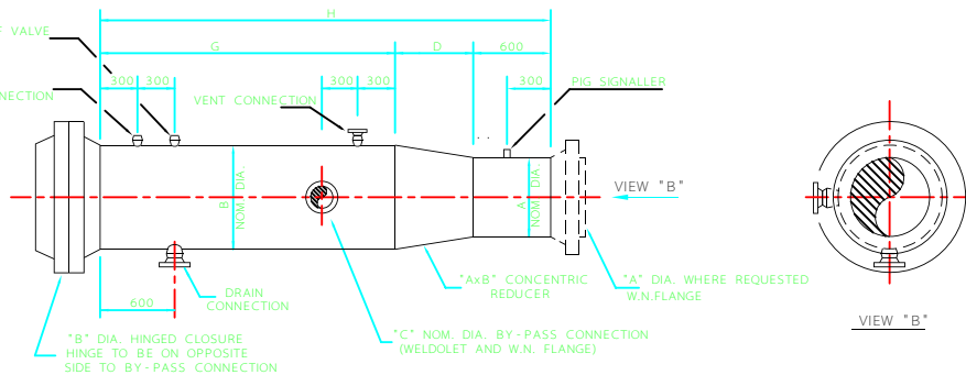
ELEVATION OF SCRAPER RECEIVING TRAP
