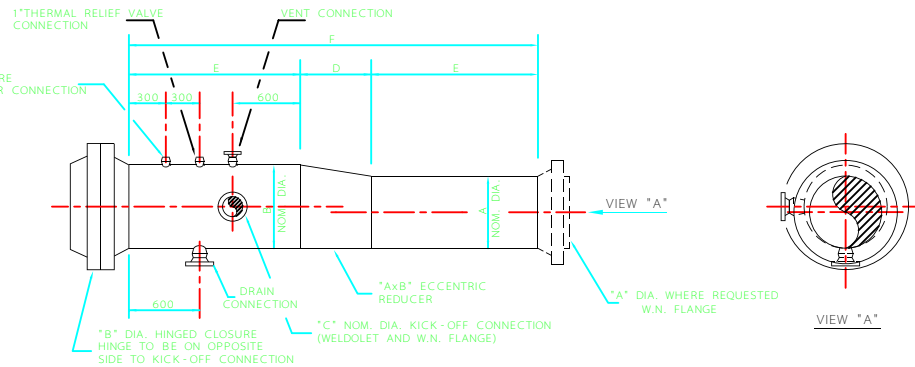
ELEVATION OF SCRAPER LAUNCHING TRAP
