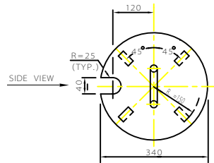
COVER PLAN DETAIL
