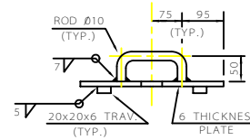
COVER SIDE VIEW
