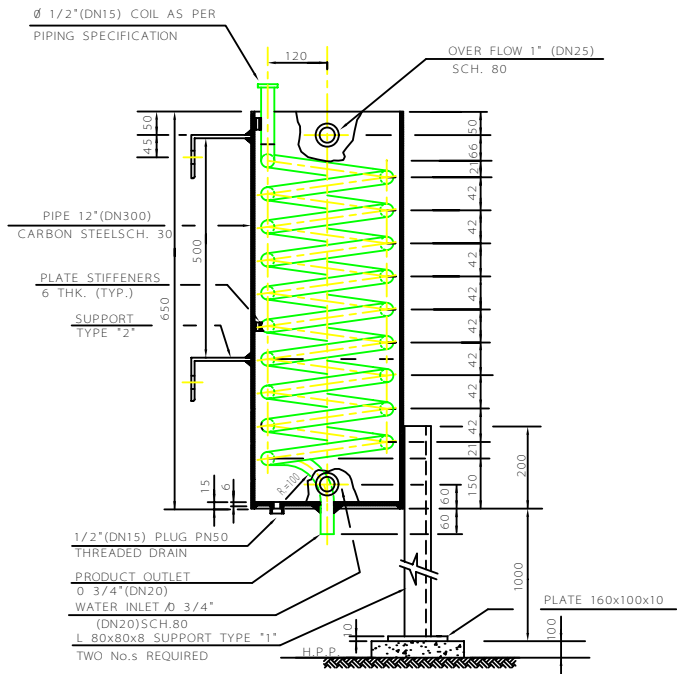
SAMPLE COOLER DETAIL
