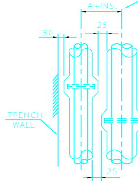
EXAMPLE III INSULATED LINES AND FLANGES
