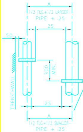
EXAMPLE I UNINSULATED LINES AND FLANGES
