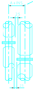
EXAMPLE II INSULATED LINES UNINSULATED FLANGES
