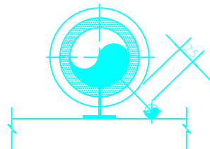
EXAMPLE V INSULATED LINES UNINSULATED FLANGES SEE NOTE 2 TO CALCULATE SPACING
