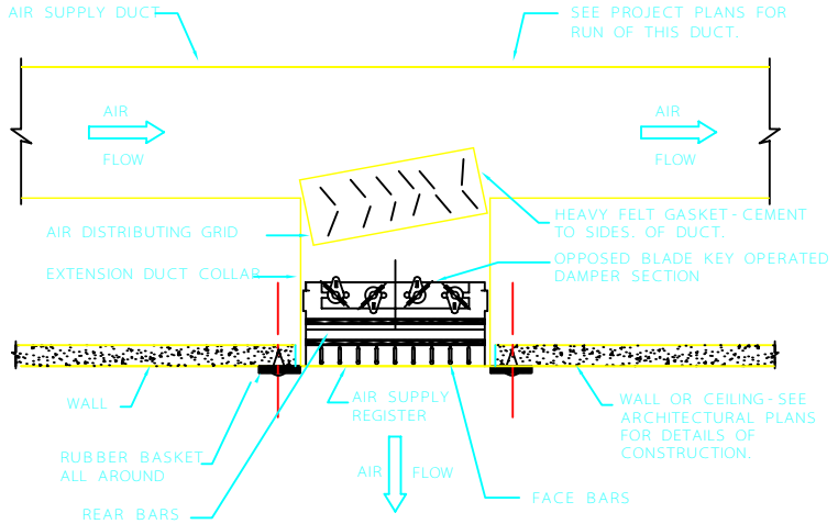
HORIZONTAL CROSS - SECTION
