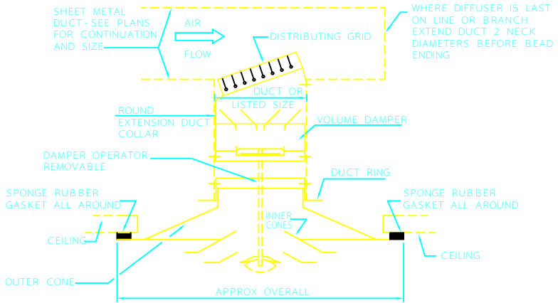
SQUARE DIFFUSER WITH ROUND NECK ADJUSTABLE PATTERN
