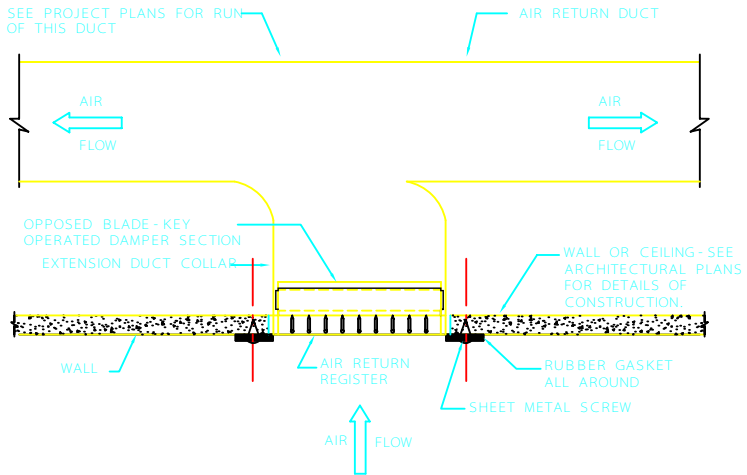
HORIZONTAL CROSS - SECTION
