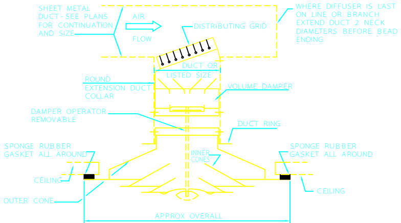
ROUND DIFFUSER WITH ROUND NECK ADJUSTABLE PATTERN
